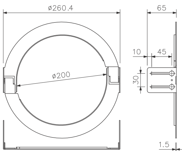
Ceiling reinforcement ring (accessory)
