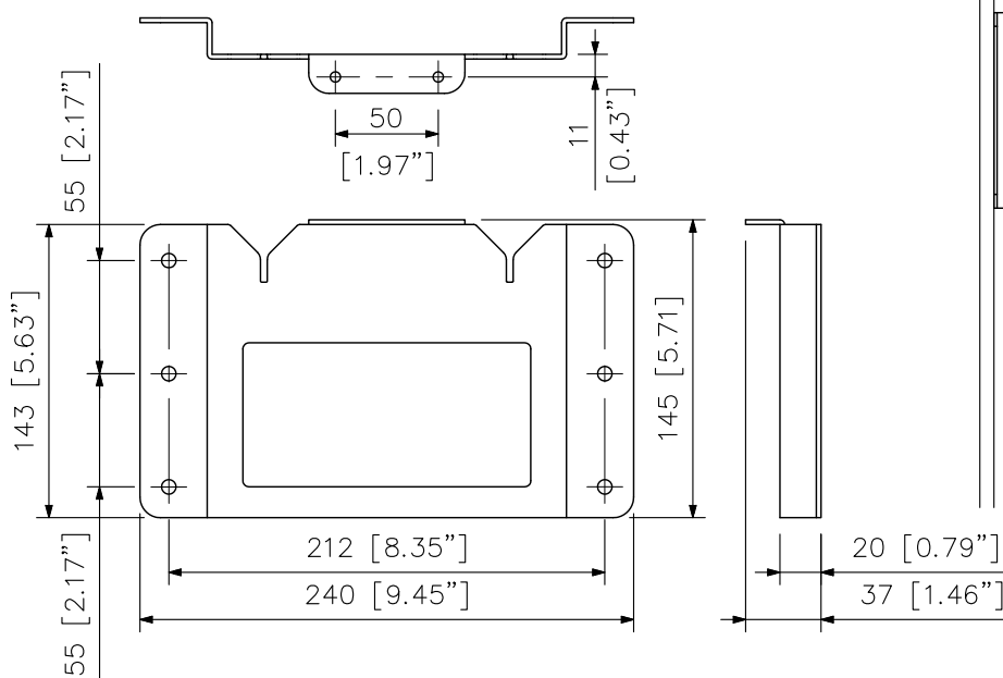
Wall bracket
