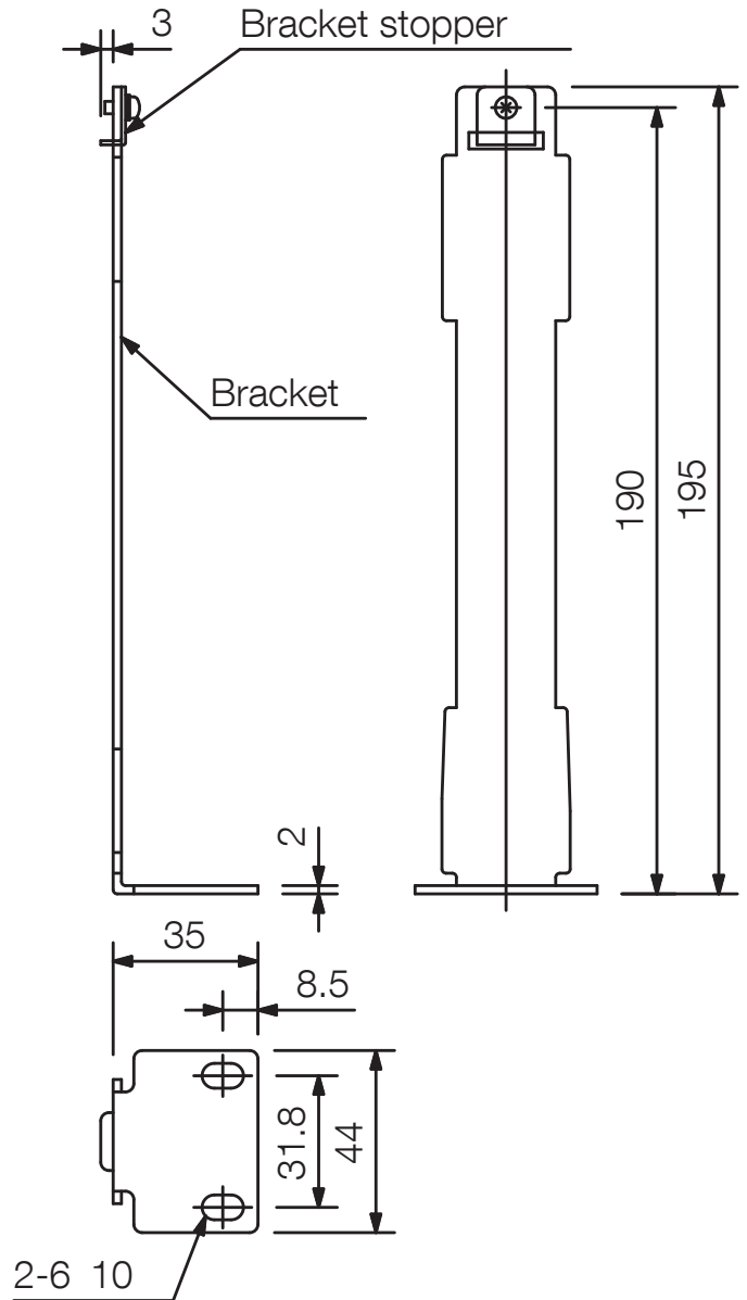
Bracket + Bracket stopper
