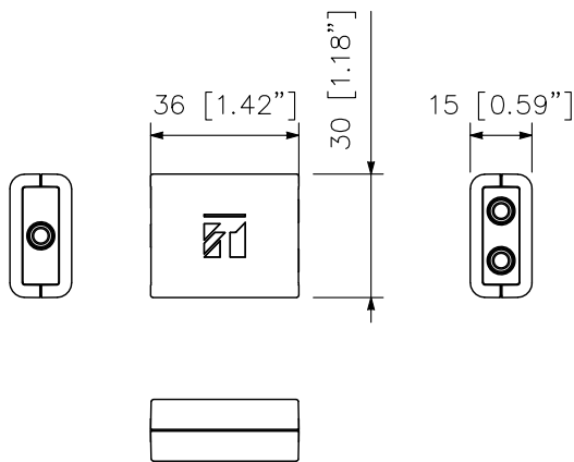
Distributor
