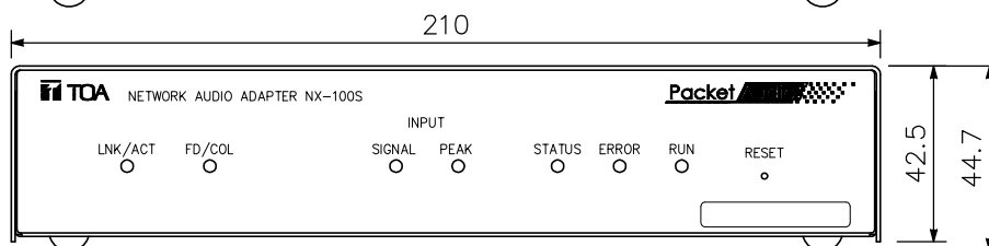
Front View
