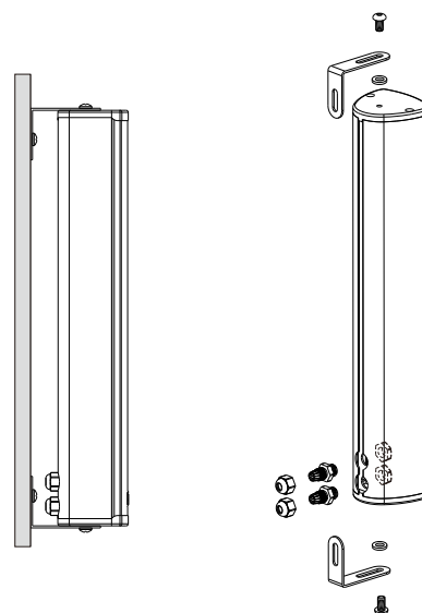
Installation drawing SCALE:1/8
