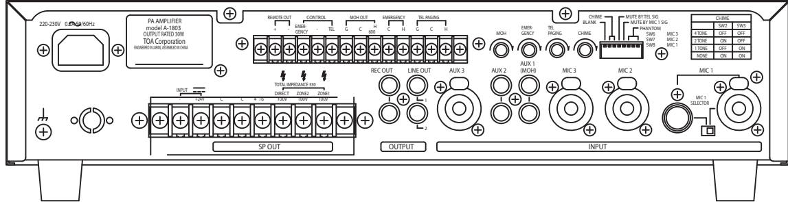
Rear View
