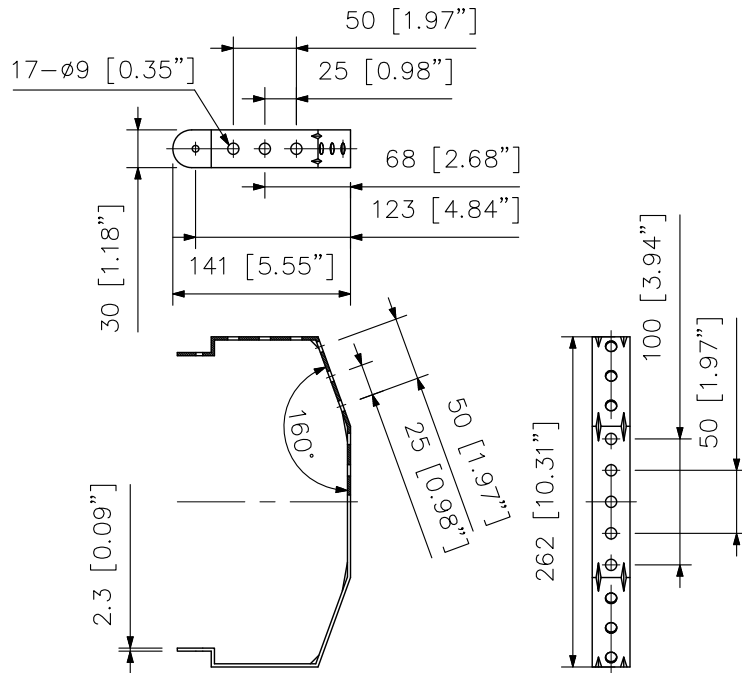
Bracket (accessory)
