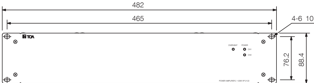
Front View
